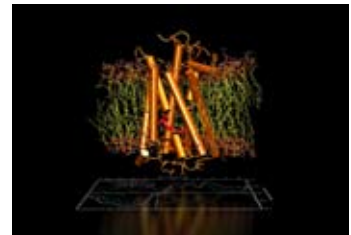
MOLECULAR DYNAMICS
